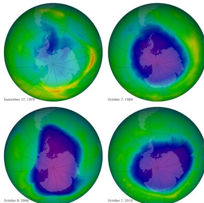
Figure (3) Recovery in the ozone layer since 1979 / NASA [7]
