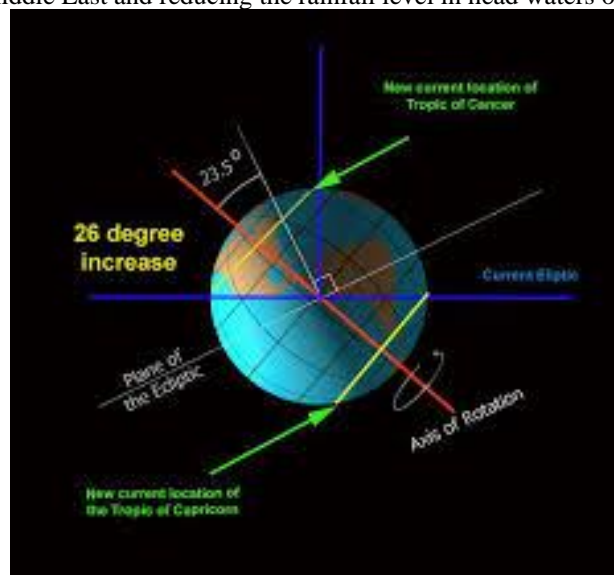
Figure (1): Shifts in earth's axis
