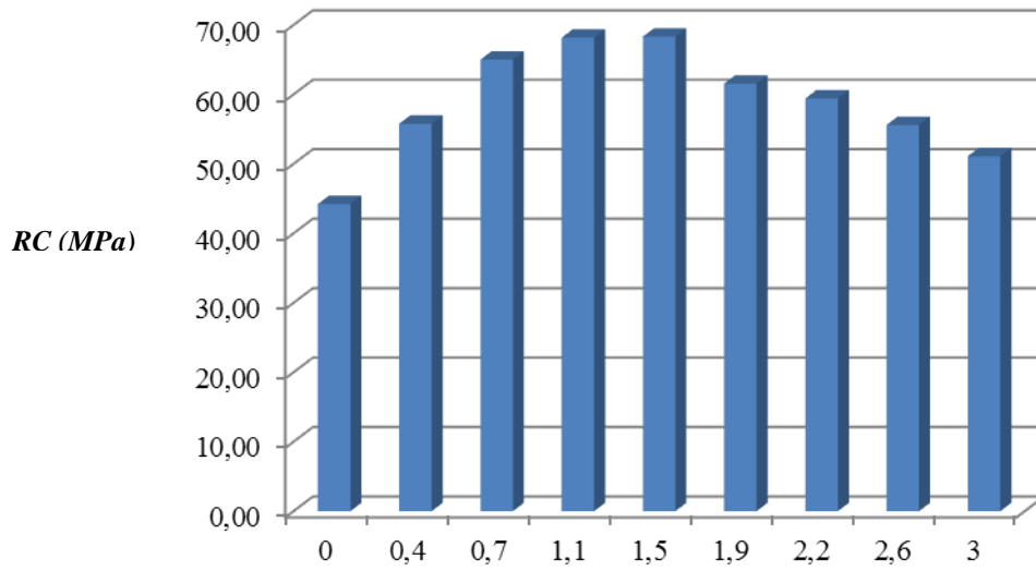
Figure 1. Compressive strength (MPa).
